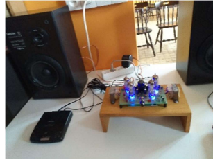
Complete opstelling
